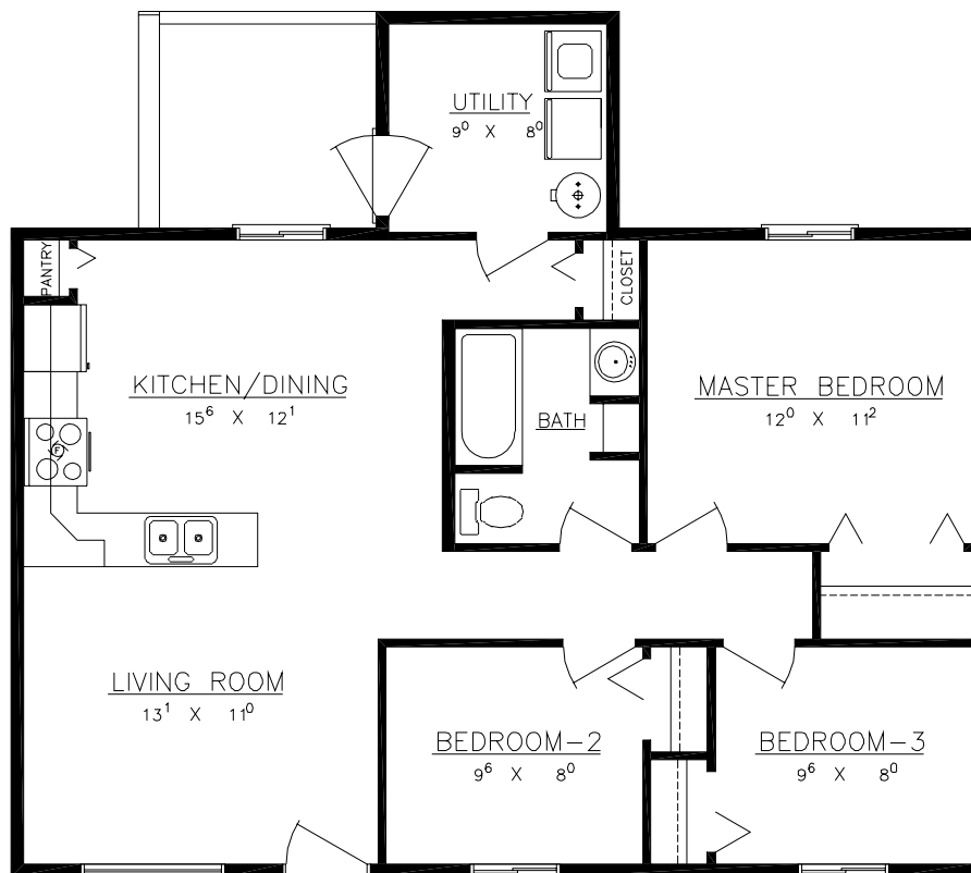
FLOOR PLAN
